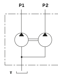
Hydraulic circuit
