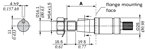
Shaft dimension
