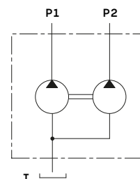
Hydraulic circuit
