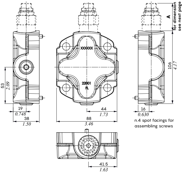
Configuration C3V dimensions
