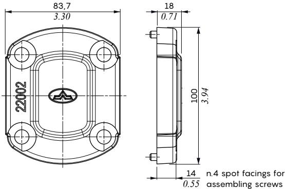
Connection position 0
