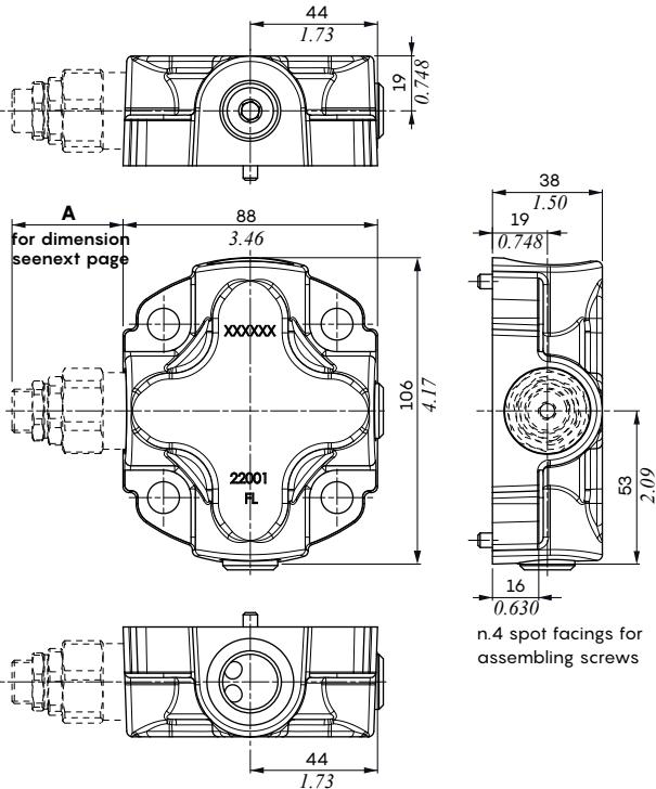
Configuration C4 dimensions
